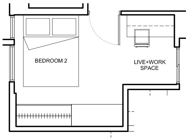
UNIT TYPE B2 - LIVE+WORK SPACE LAYOUT A
